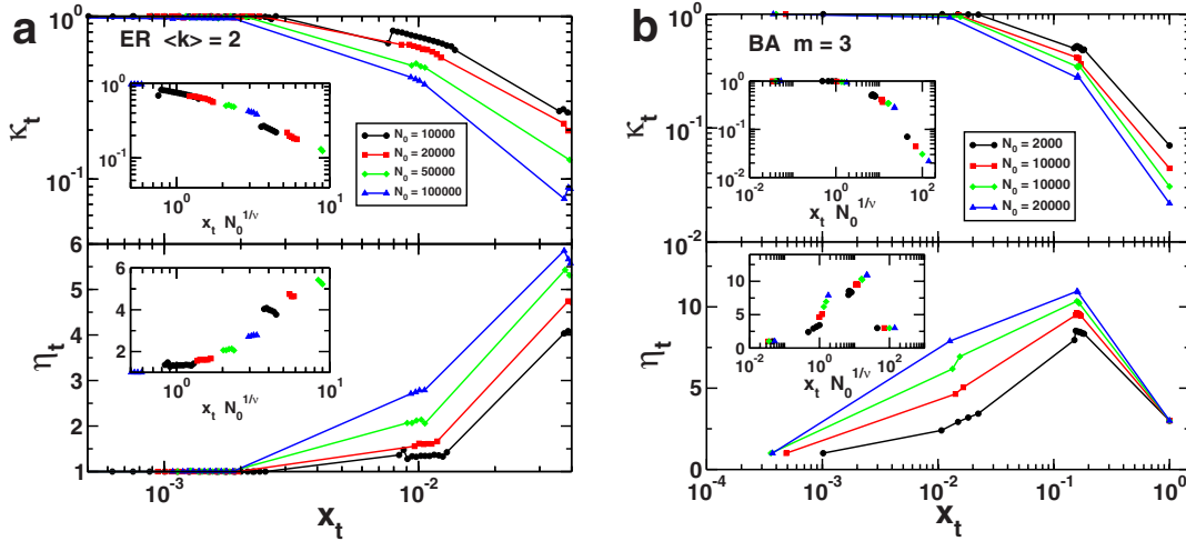
FIG. 7. (Color online) Study of renormalization flows on non-self-similar artificial graphs. Renormalization has been performed by using GCA with \ell_B=3 . The figures display the variables \kappa_t (a,b top) and \eta_t (a,b bottom) as a function of the relative network size x_t , for the renormalization flow of an ER model with \langle k \rangle=2 (a) and a BA model with 2m=\langle k \rangle=6 (b). The insets display the scaling function of the variable (x_t-x^*)N_0^{1/\nu} for \kappa_t and \eta_t . Here the scaling exponent is \nu=2 in both cases.
