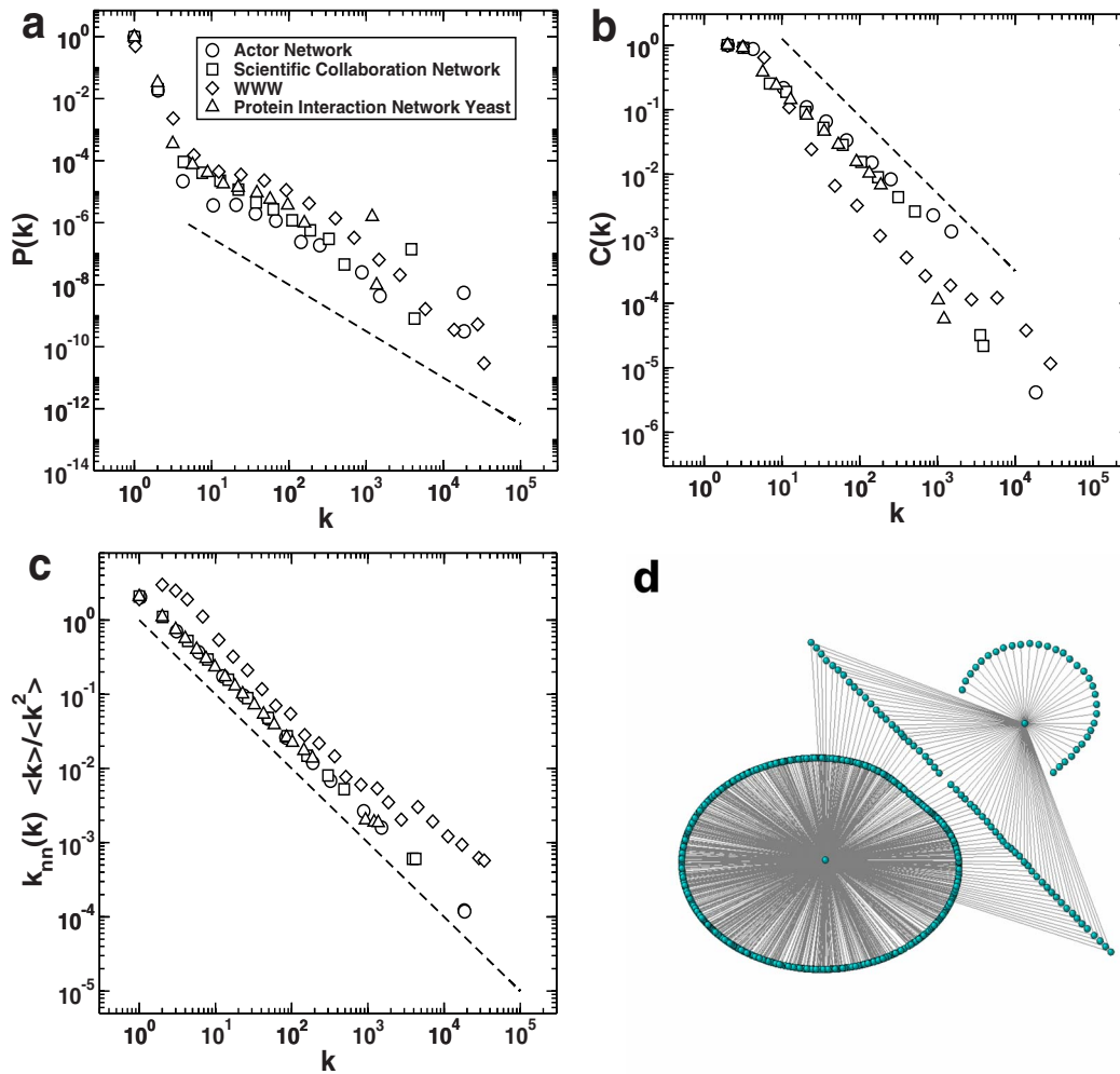
FIG. 11. (Color online) Statistical properties of the “fixed point” in the case of real networks. Renormalization has been performed by using GCA with \ell_B=2 . The properties of the networks are measured after a certain number (less than 10) of renormalization steps. Dashed lines have the same slopes as those appearing in Fig. 6. The real networks considered in this figure are the actor network [8], the scientific collaboration network [30], the network of Web pages of the domain of the University of Notre Dame [26], and the protein-protein interaction network of the yeast Saccharomyces cerevisiae [31]. (d) The graphical representation of the fixed point has been obtained by starting from the protein-protein interaction network of the yeast.
