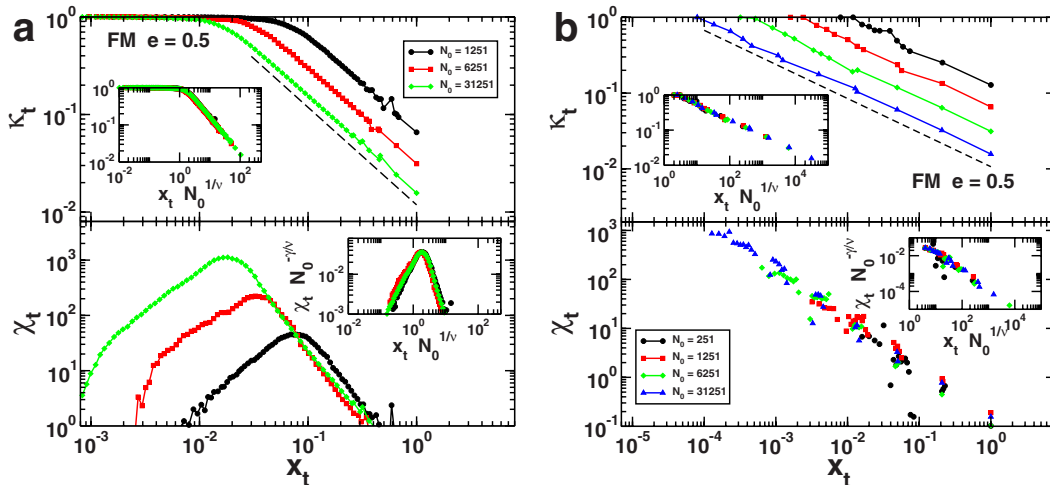
FIG. 8. (Color online) Study of renormalization flows on self-similar artificial graphs. The box covering has been performed by using RB with r_B=1 (a) and GCA with \ell_B=3 (b). The graph is an FM network with e=0.5 , where e is the probability for hub-hub attraction [13]. The figures display \kappa_t (a,b, top), and \chi_t (a,b, bottom) as a function of the relative network size x_t . The scaling function of the variable (x_t-x^*)N_0^{1/\nu} for \kappa_t and \chi_t is displayed in the insets. We find that the two box covering techniques yield different exponent values: \nu=2.2 (RB) and \nu=1 (GCA). The dashed lines indicate the predicted behavior of the scaling function. In (a) the exponent of the power law decay for the scaling function is -1 , independently of the exponent \beta of the degree distribution of the initial graph; in (b) instead the scaling function decays with an exponent -(\beta-2)/(\beta-1)=-0.45 . We still find \gamma=\nu for both transformations.
