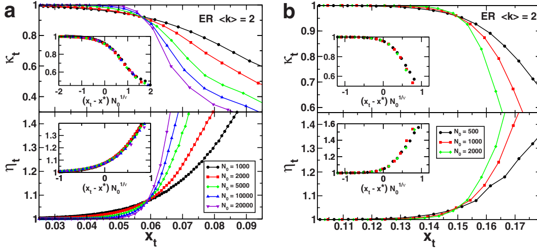
FIG. 2. (Color online) Study of renormalization flows on the ER model with \langle k \rangle = 2 . The box covering has been performed by using RB with r_B = 1 (a) and GCA with \ell_B = 2 (b). The figures display \kappa_t (a, b top) and \eta_t (a, b bottom) as a function of the relative network size x_t . The insets display the scaling function of the variable (x_t - x^*) N_0^{1/\nu} for \kappa_t and \eta_t . Here the scaling exponent \nu = 2 in both cases. Note that the flow of the renormalization procedure goes from larger (right on the x axis) to smaller values (left) of x_t .
